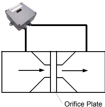
Orifice Plate (differential pressure)
