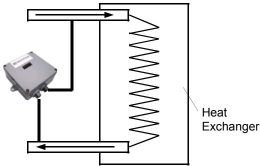
Plate Heat Exchanger (differential pressure)
